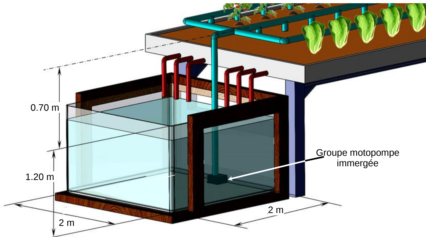
Figure 9 : station aquaponique
