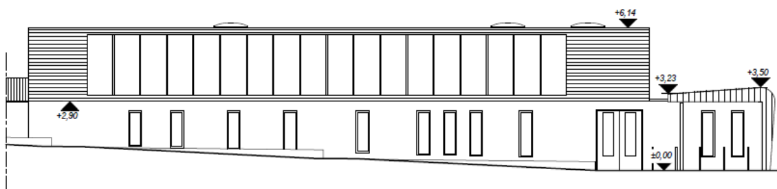
Façade principale
