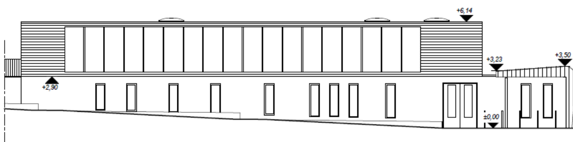
Façade principale
